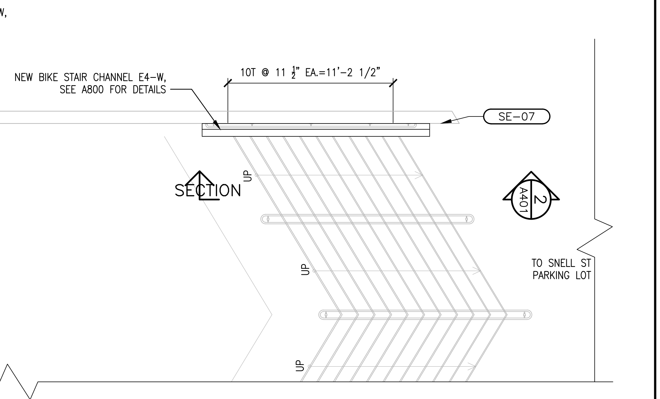
1 COLISEUM STATION STAIR E4 PARTIAL PLAN A401 SCALE: 1/4" = 1'-0"
