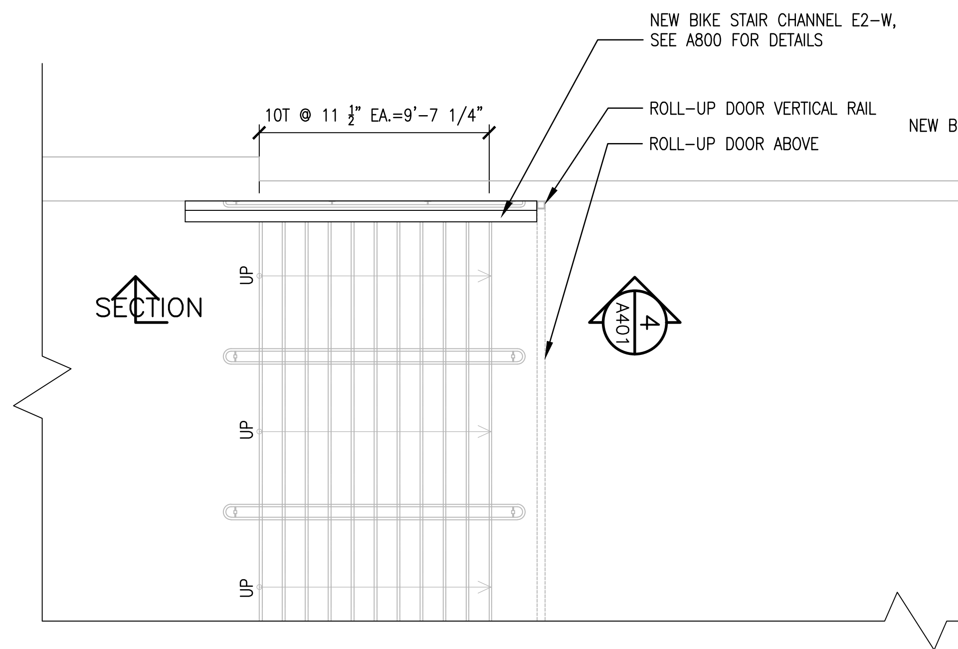
3 COLISEUM STATION STAIR E2 PARTIAL PLAN A401 SCALE: 1/4" = 1'-0"
