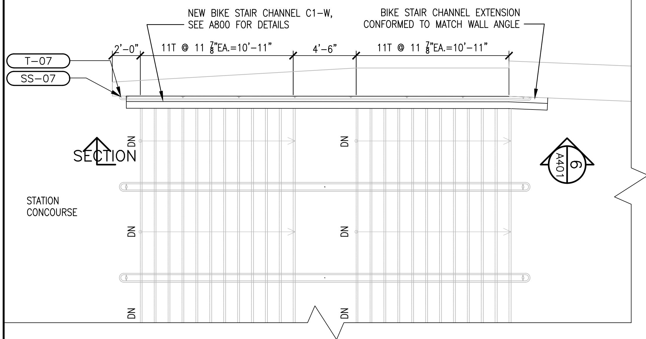
5 COLISEUM STATION STAIR C1 PARTIAL PLAN A401 SCALE: 1/4" = 1'-0"
