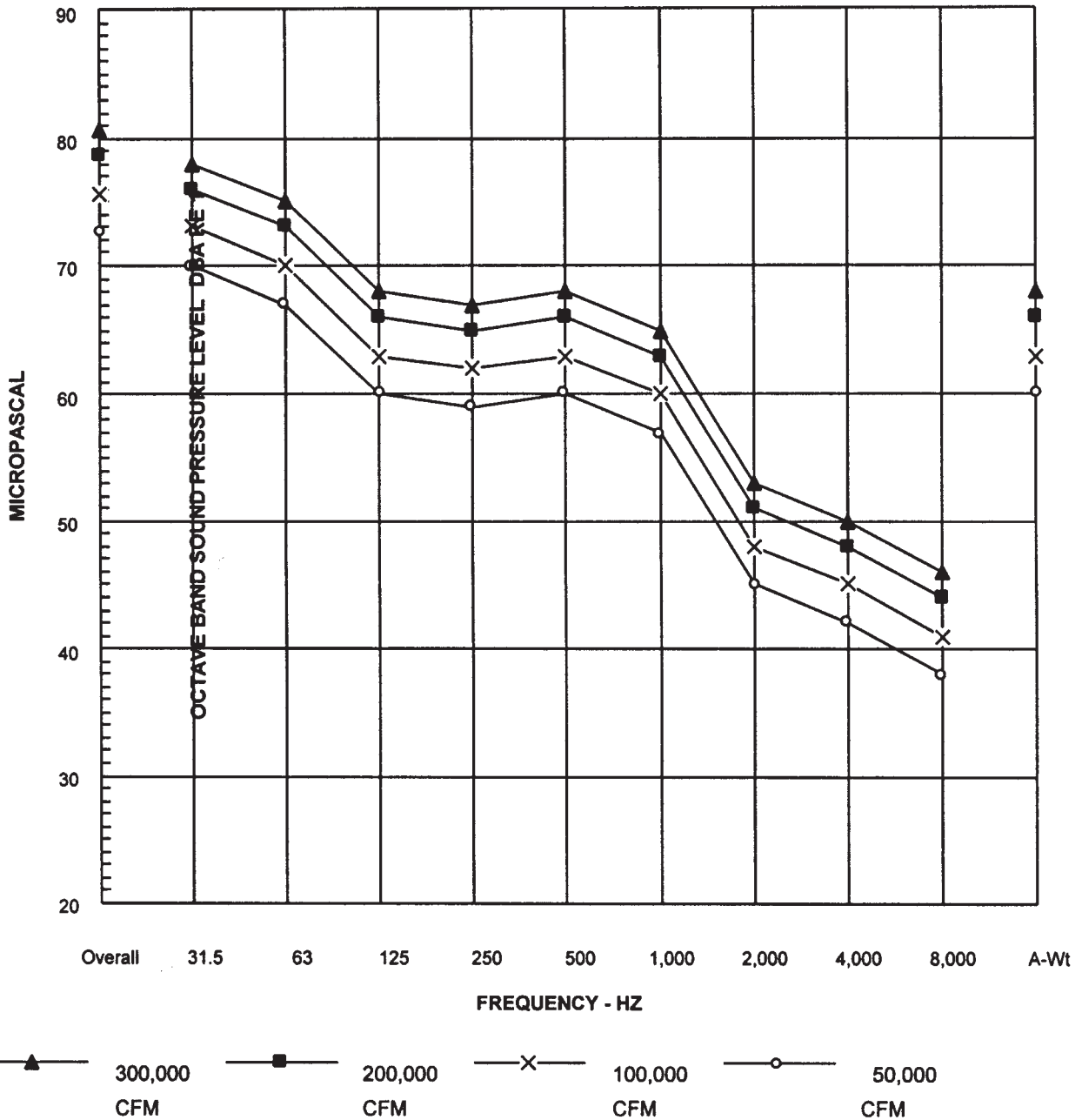
FIGURE 9-13 WMATA DESIGN CURVES FOR MAXIMUM EXPECTED TRAIN NOISE AT 30 FEET FROM SHAFT GRATINGS
