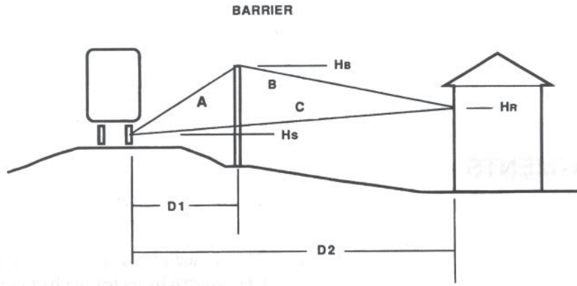
FIGURE 9-1 SOUND BARRIER SOURCE-PATH-RECEIVER RELATIONSHIP
