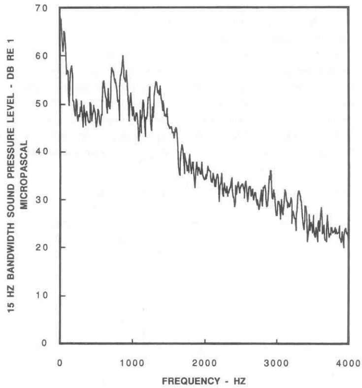
FIGURE 2-9 EXAMPLE OF FOURIER SPECTRAL ANALYSIS
