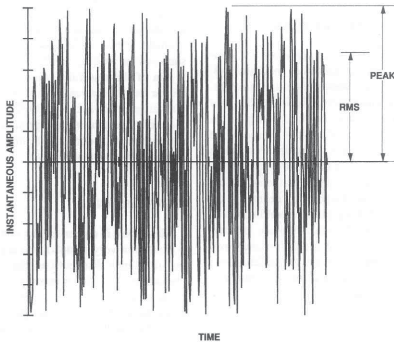
FIGURE 2-4 RANDOM WAVEFORM EXAMPLE
