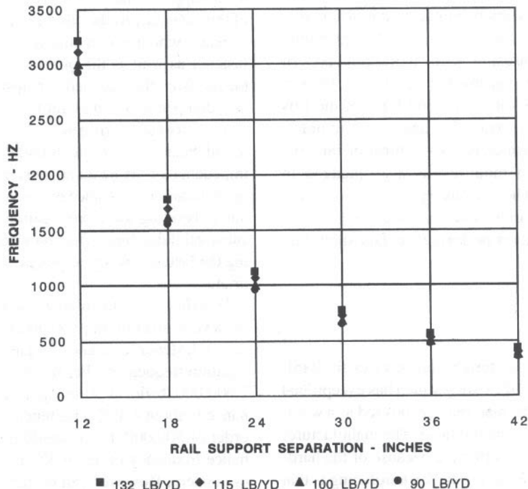
FIGURE 10-4 VERTICAL PINNED-PINNED RESONANCE FREQUENCY VS. RAIL SUPPORT SEPARATION FOR VARIOUS RAILS
