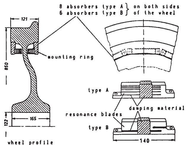
FIGURE 7-8 KRUPP TUNED VIBRATION ABSORBER
