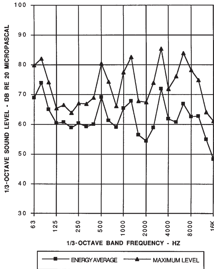
FIGURE 4-19 WHEEL SQUEAL AT PORTLAND TRI-MET WITH RESILIENT BOCHUM WHEELS ON URETHANE EMBEDDED TRACK WITH 87-FOOT RADIUS CURVE
